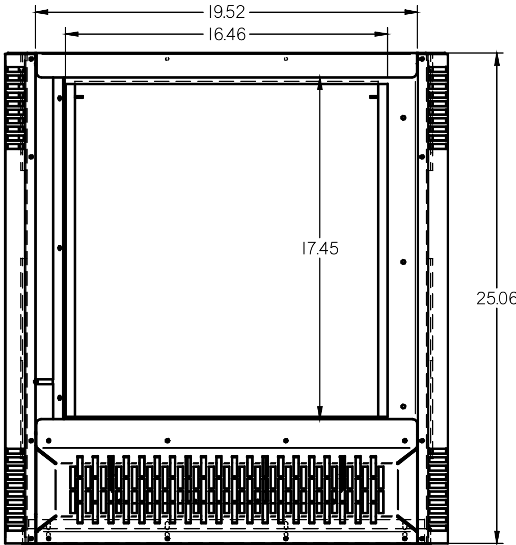
MODEL I6090: COLORAM II - LARGE FORMAT
